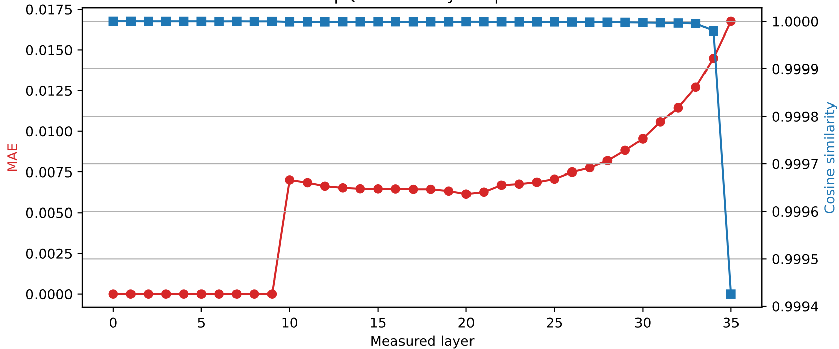
SmolLM3-3B | Quantized layer 9 | float32 \rightarrow int8
