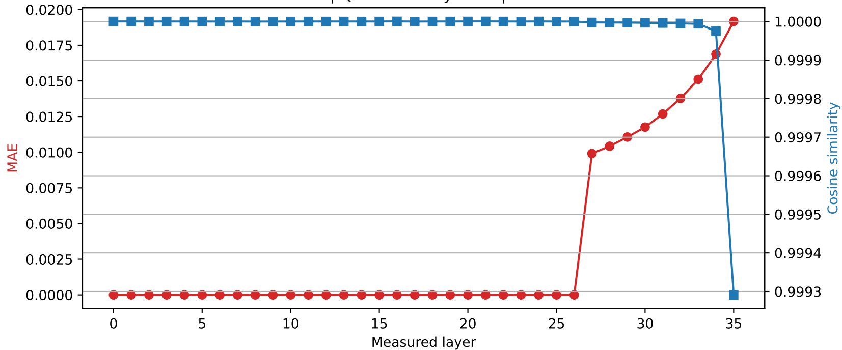
SmolLM3-3B | Quantized layer 26 | float32 → int8
