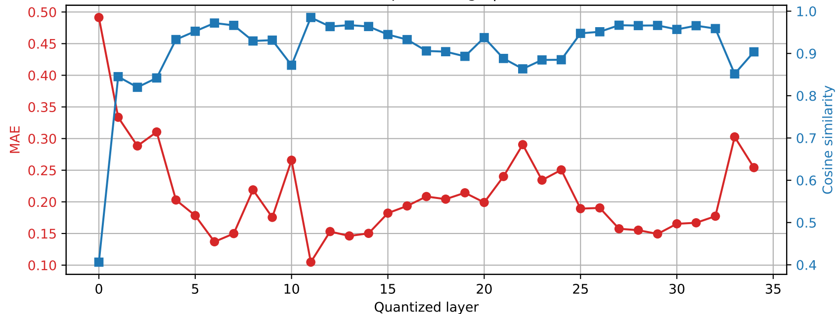
SmolLM3-3B | Prompt 0 Final RMSNorm output damage | float32 \rightarrow int4
