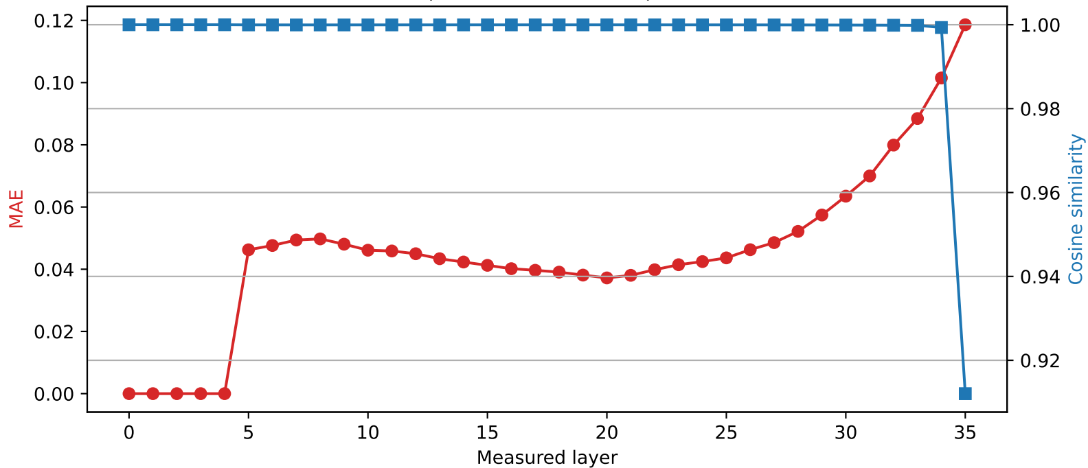
SmolLM3-3B | Quantized layer 4 | float32 → int4
