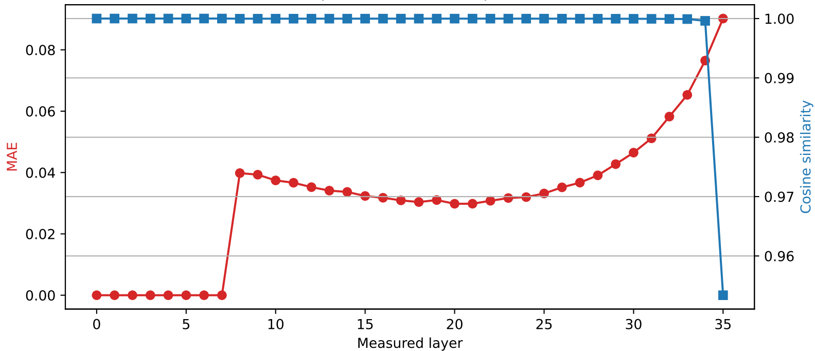
SmolLM3-3B | Quantized layer 7 | float32 \rightarrow int4
