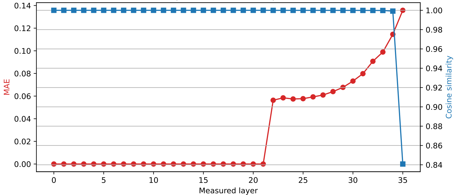
SmolLM3-3B | Quantized layer 21 | float32 \rightarrow int4
