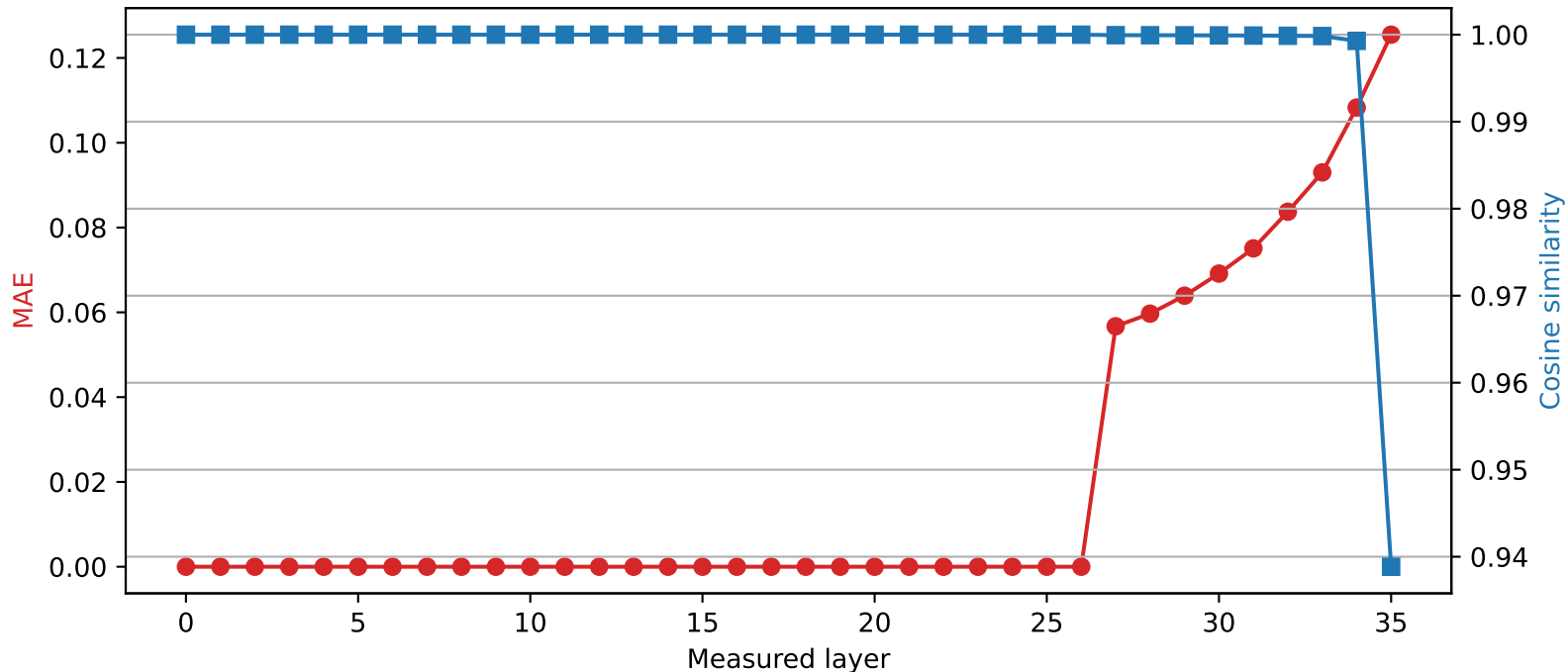
SmolLM3-3B | Quantized layer 26 | float32 → int4
