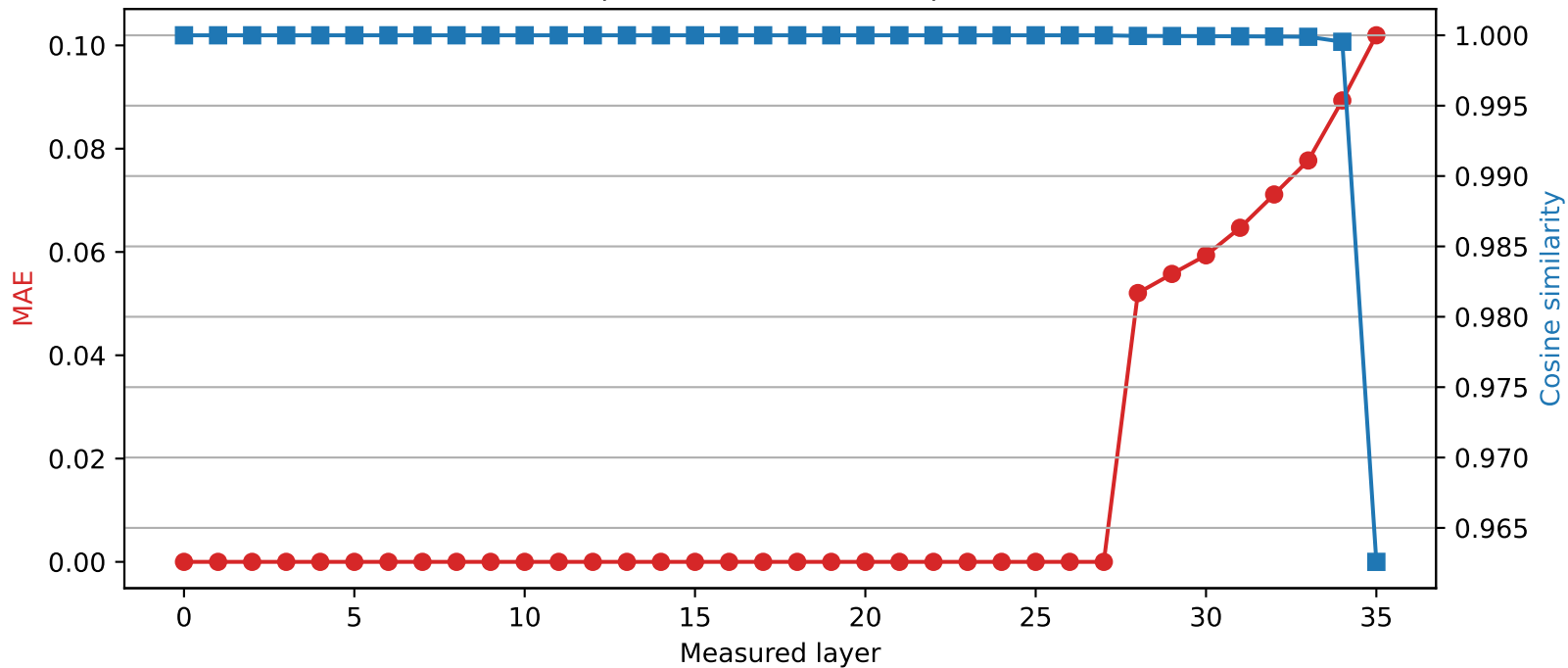
SmolLM3-3B | Quantized layer 27 | float32 \rightarrow int4
