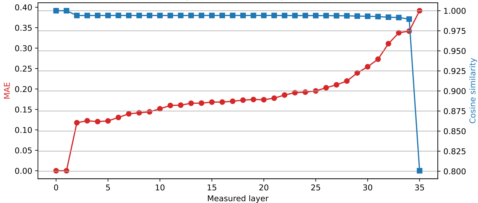
SmolLM3-3B | Quantized layer 1 | float32 \rightarrow int4
