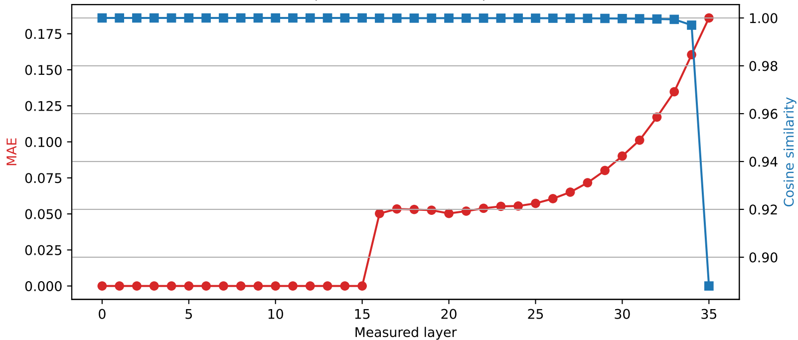
SmolLM3-3B | Quantized layer 15 | float32 → int4
