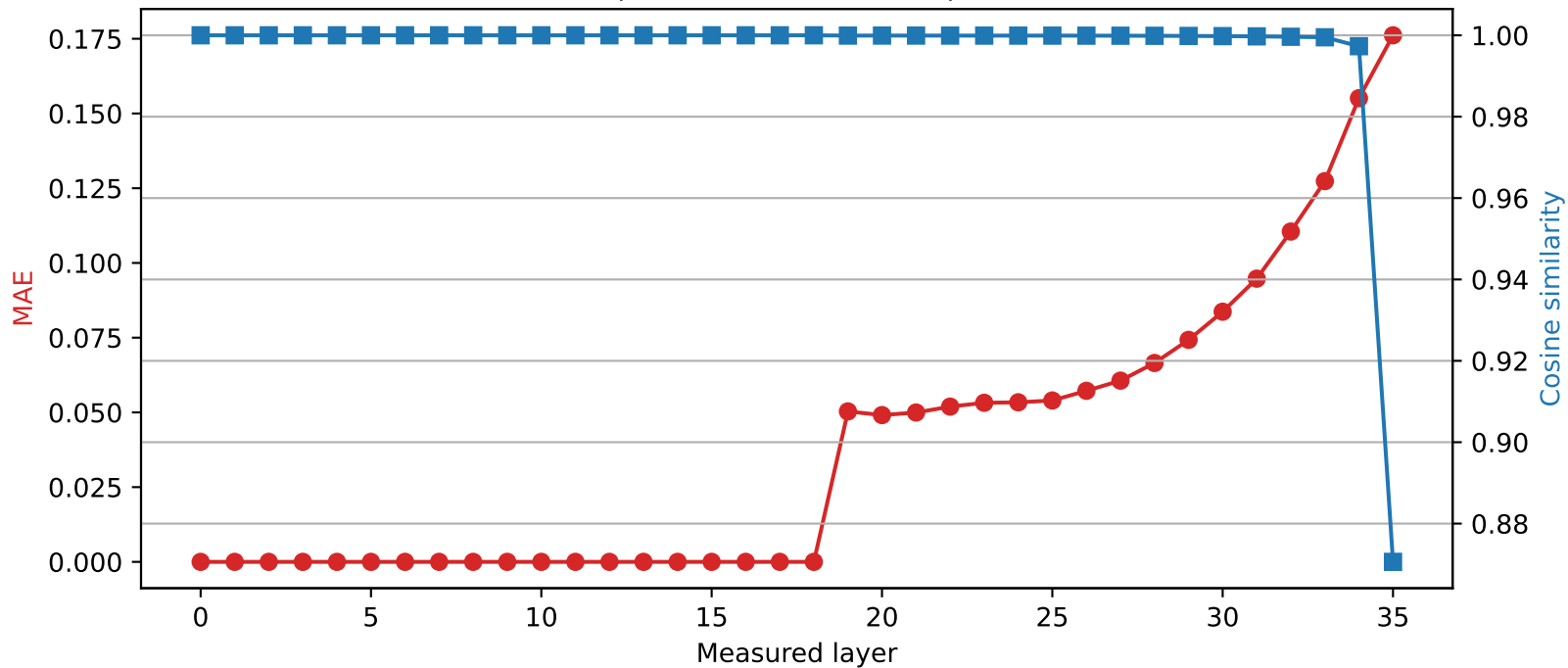
SmolLM3-3B | Quantized layer 18 | float32 \rightarrow int4
