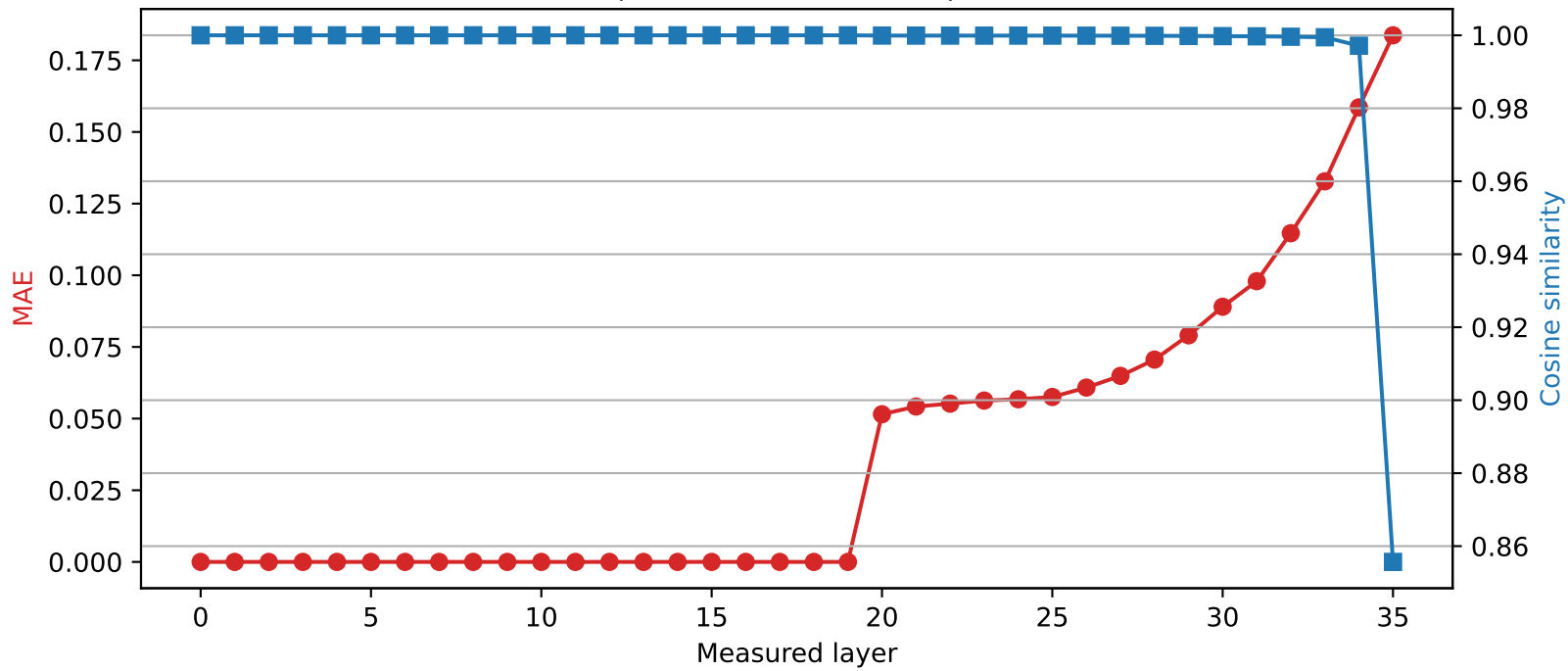
SmolLM3-3B | Quantized layer 19 | float32 \rightarrow int4
