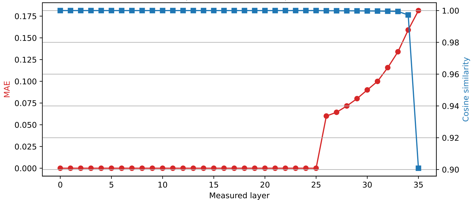
SmolLM3-3B | Quantized layer 25 | float32 \rightarrow int4
