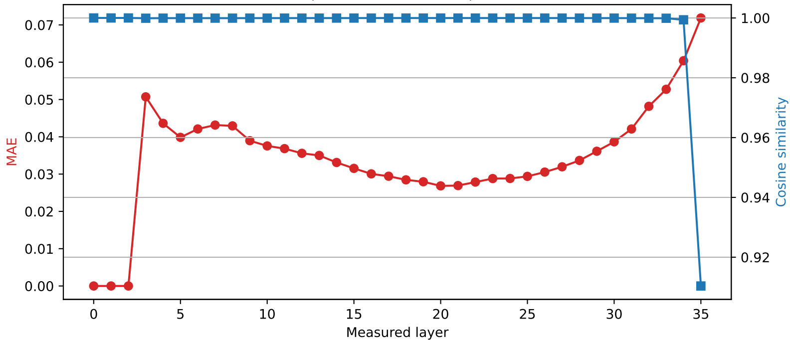
SmolLM3-3B | Quantized layer 2 | float32 → int4
