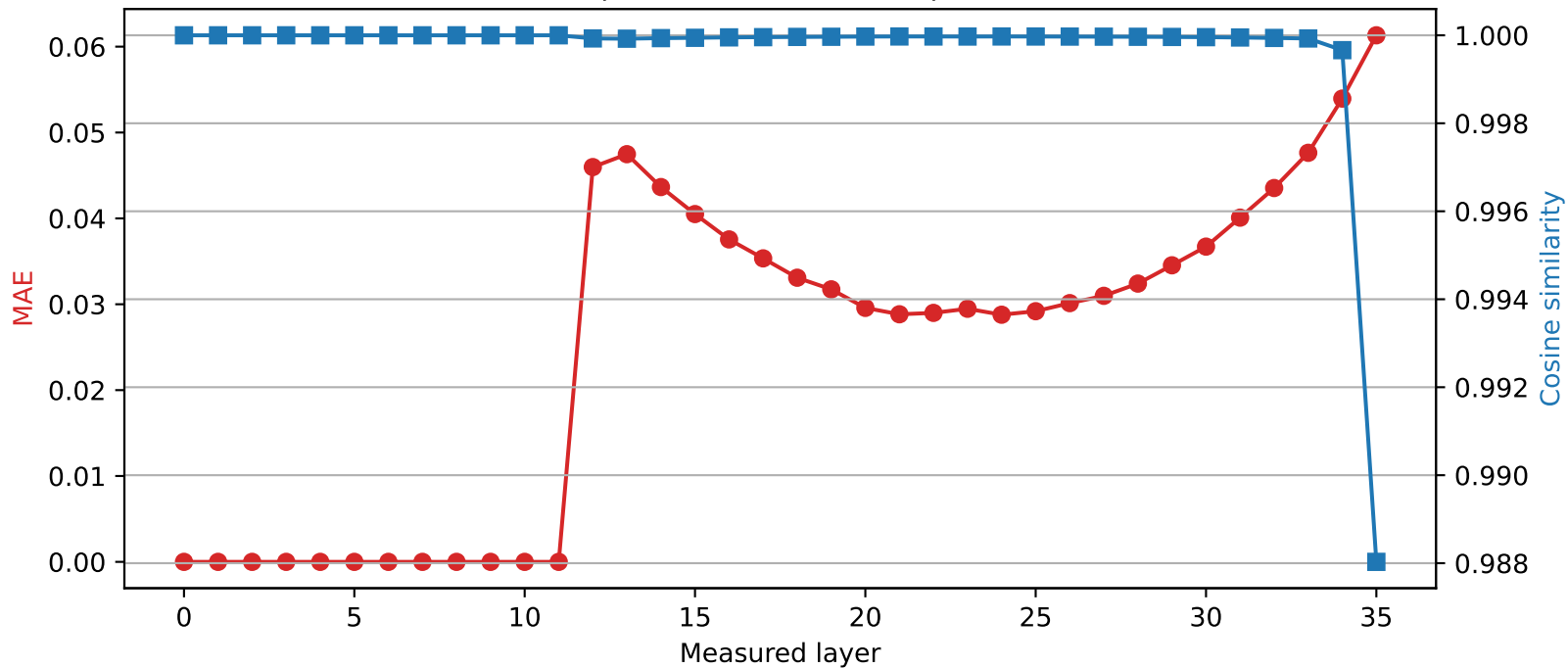
SmolLM3-3B | Quantized layer 11 | float32 \rightarrow int4
