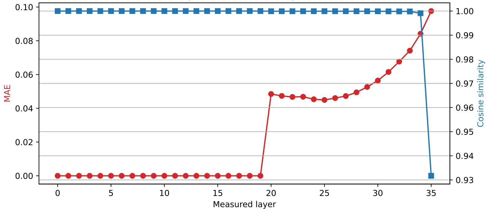
SmolLM3-3B | Quantized layer 19 | float32 → int4
