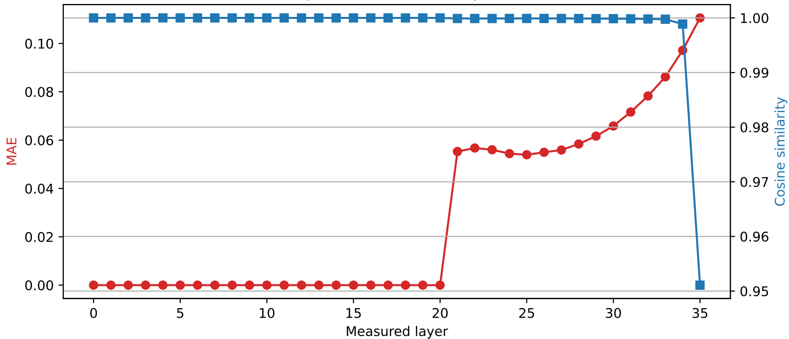
SmolLM3-3B | Quantized layer 20 | float32 \rightarrow int4
