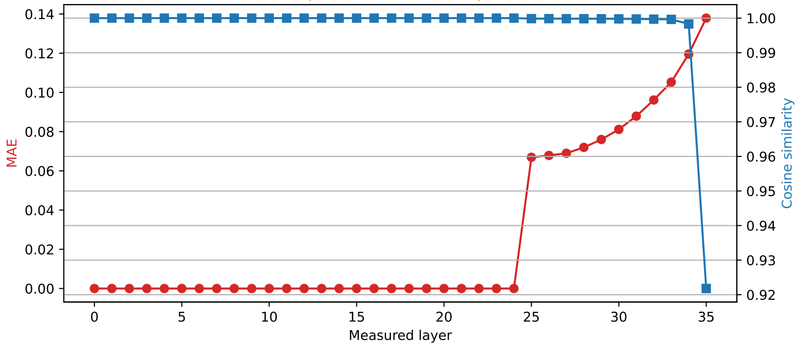
SmolLM3-3B | Quantized layer 24 | float32 \rightarrow int4
