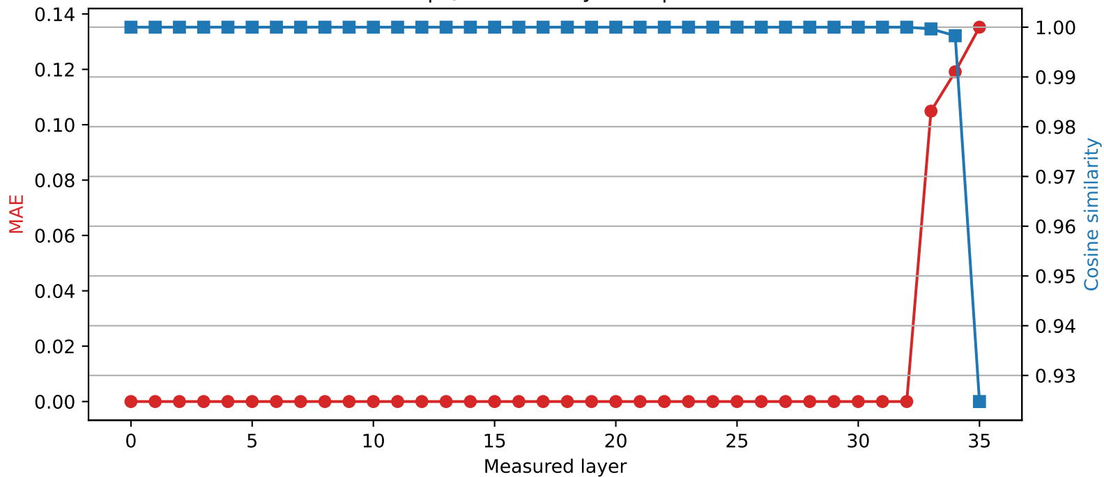
SmolLM3-3B | Quantized layer 32 | float32 \rightarrow int4
