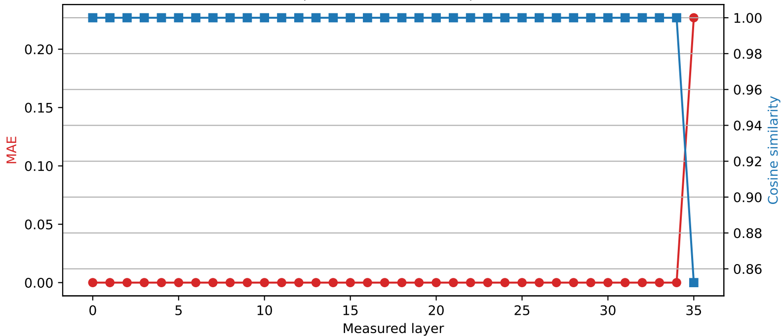
SmolLM3-3B | Quantized layer 34 | float32 \rightarrow int4
