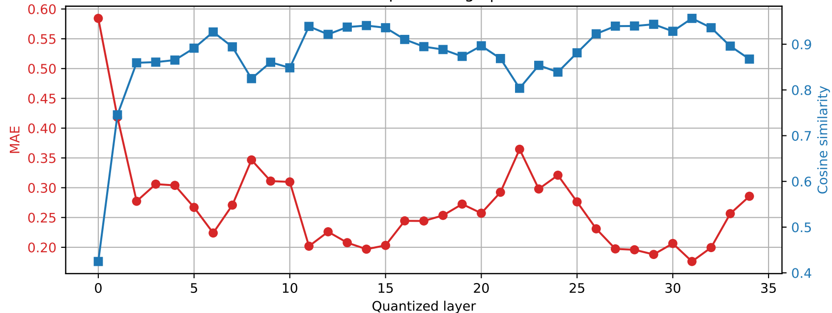
SmolLM3-3B | Prompt 3 Final RMSNorm output damage | float32 \rightarrow int4
