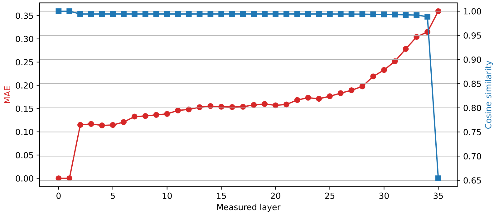
SmolLM3-3B | Quantized layer 1 | float32 → int4
