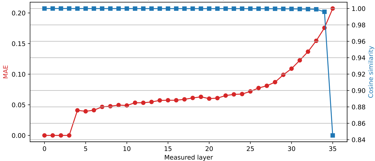
SmolLM3-3B | Quantized layer 3 | float32 \rightarrow int4
