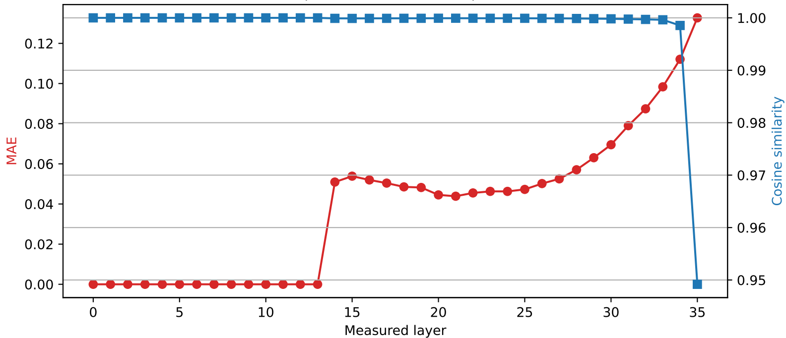
SmolLM3-3B | Quantized layer 13 | float32 \rightarrow int4
