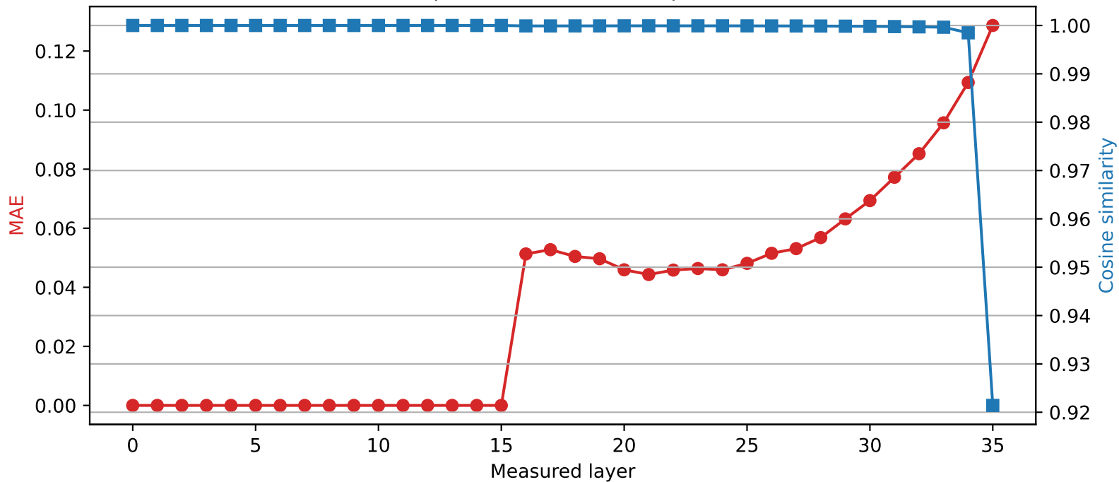
SmolLM3-3B | Quantized layer 15 | float32 \rightarrow int4
