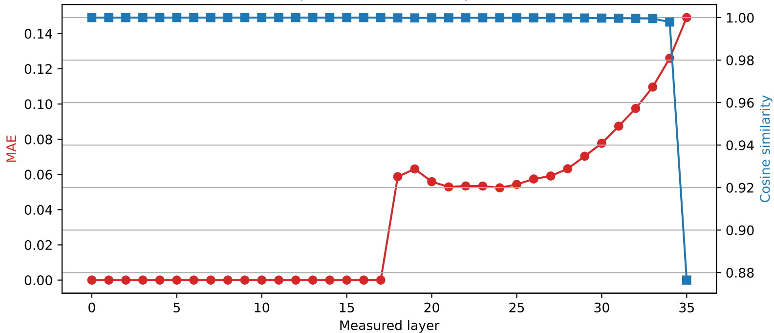
SmolLM3-3B | Quantized layer 17 | float32 \rightarrow int4
