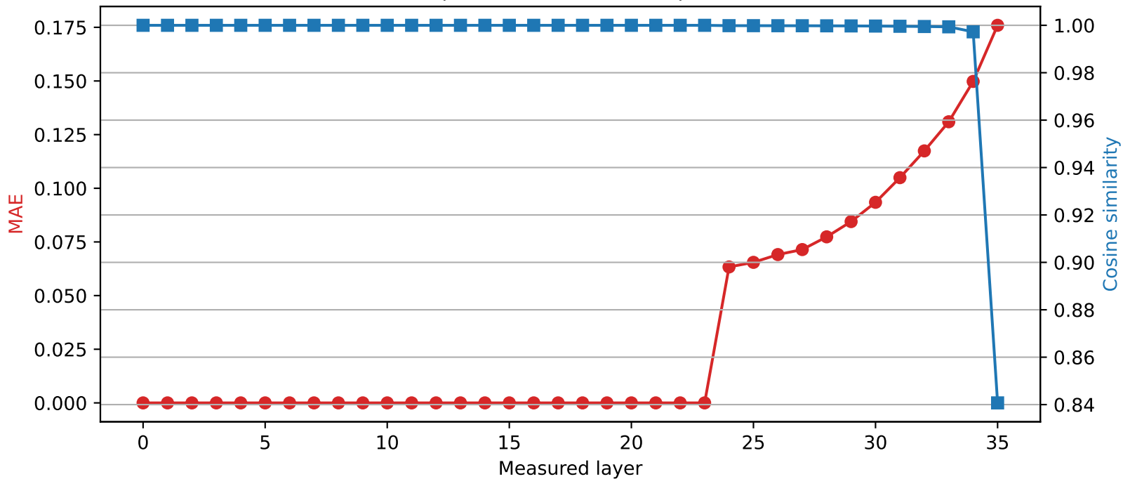
SmolLM3-3B | Quantized layer 23 | float32 → int4
