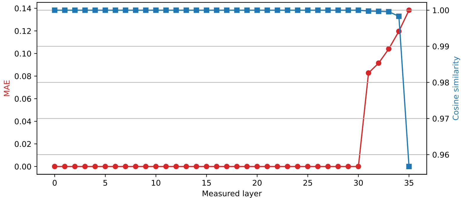
SmolLM3-3B | Quantized layer 30 | float32 \rightarrow int4
