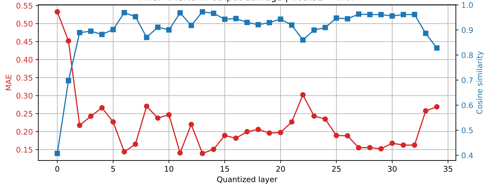
SmolLM3-3B | Prompt 4 Final RMSNorm output damage | float32 \rightarrow int4
