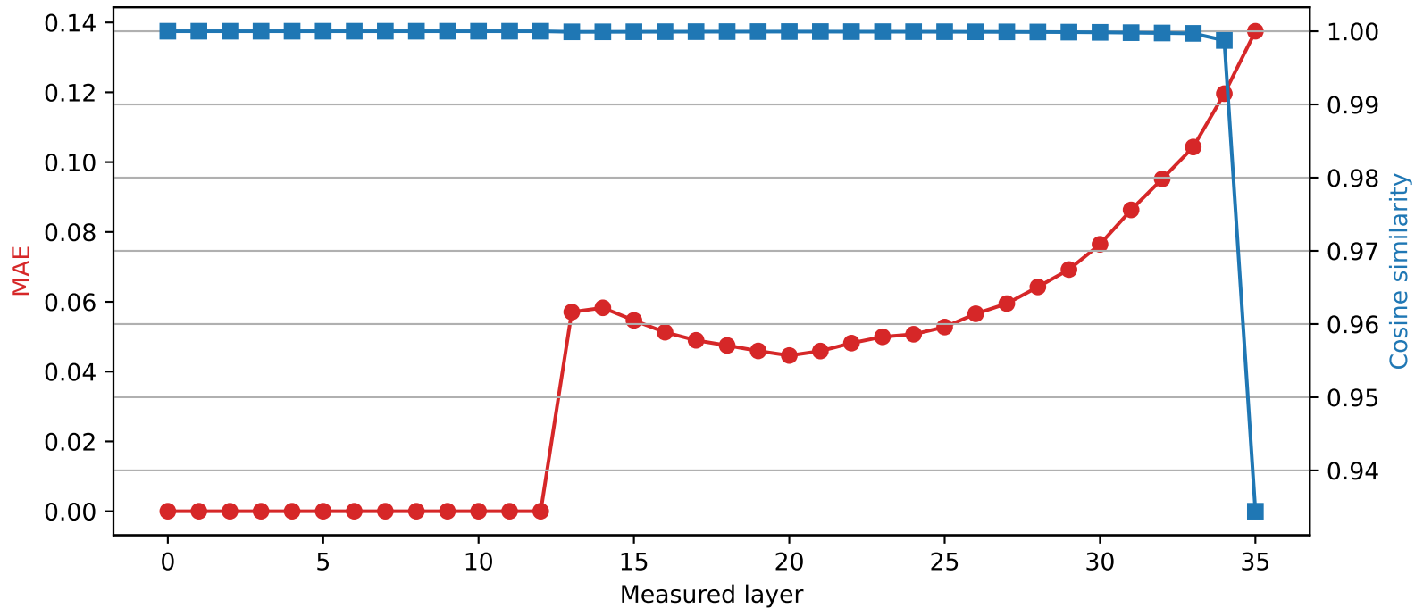
SmolLM3-3B | Quantized layer 12 | float32 → int4
