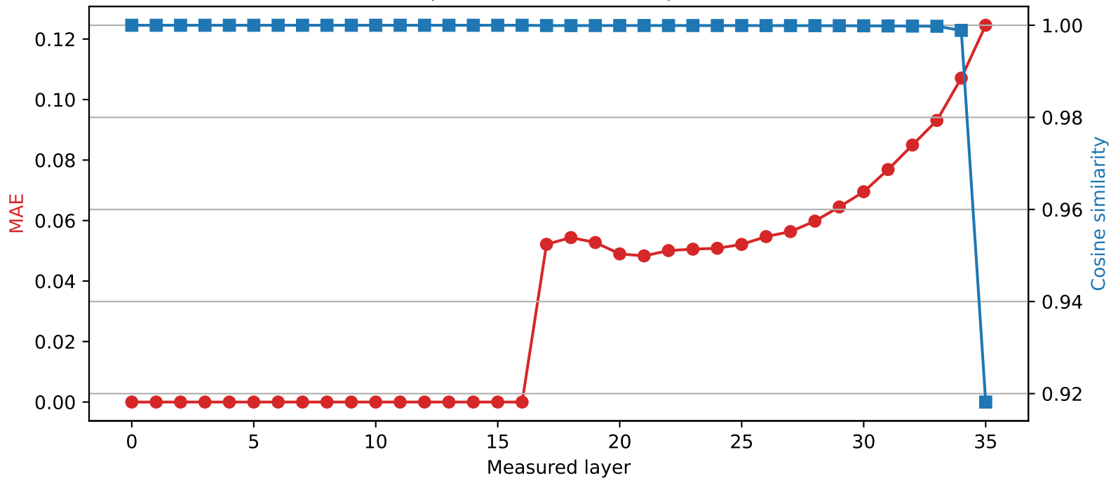
SmolLM3-3B | Quantized layer 16 | float32 \rightarrow int4
