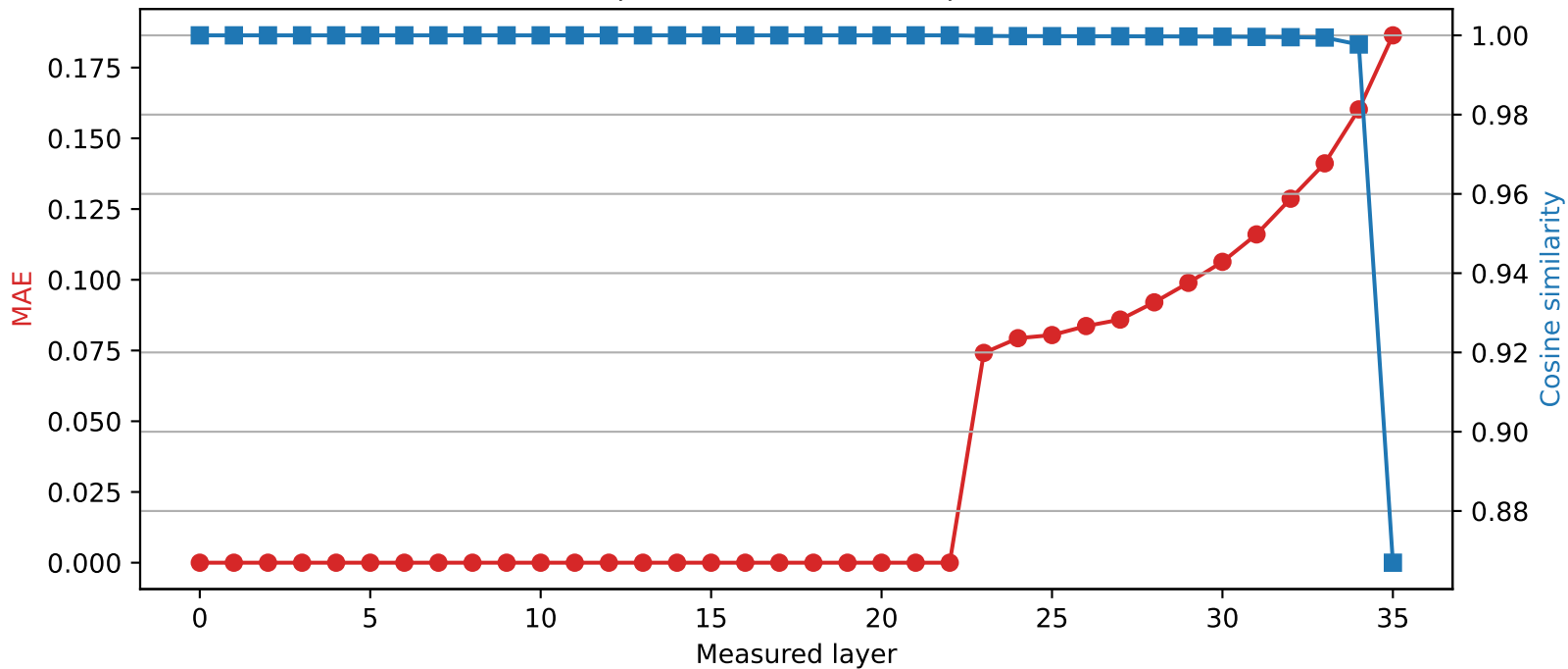
SmolLM3-3B | Quantized layer 22 | float32 \rightarrow int4
