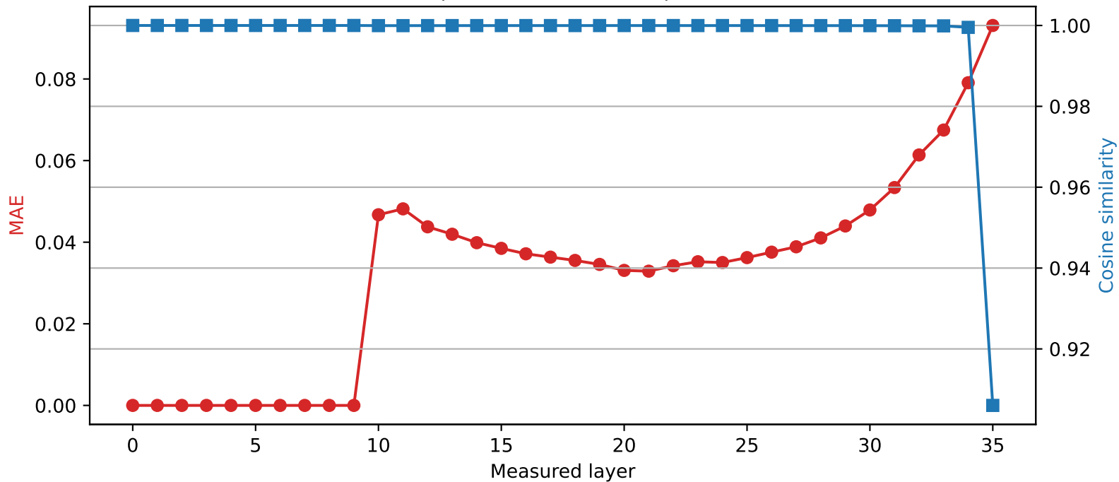
SmolLM3-3B | Quantized layer 9 | float32 \rightarrow int2
