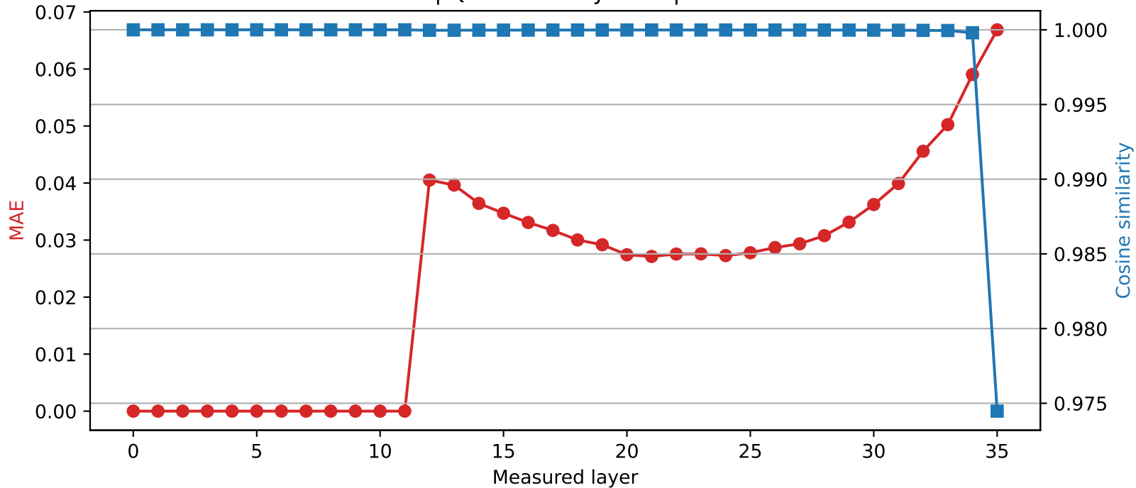
SmolLM3-3B | Quantized layer 11 | float32 → int2
