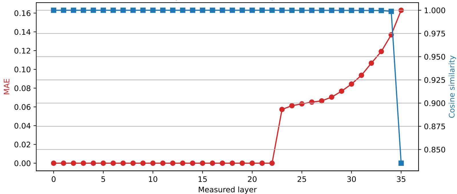
SmolLM3-3B | Quantized layer 22 | float32 \rightarrow int2
