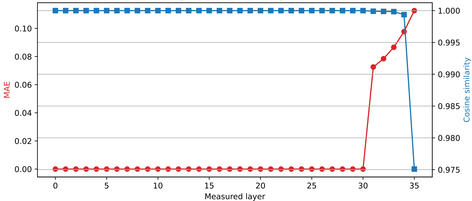
SmolLM3-3B | Quantized layer 30 | float32 → int2
