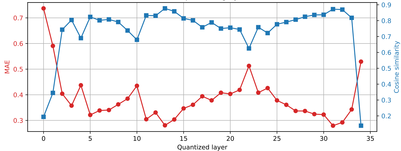
SmolLM3-3B | Prompt 1 Final RMSNorm output damage | float32 \rightarrow int2
