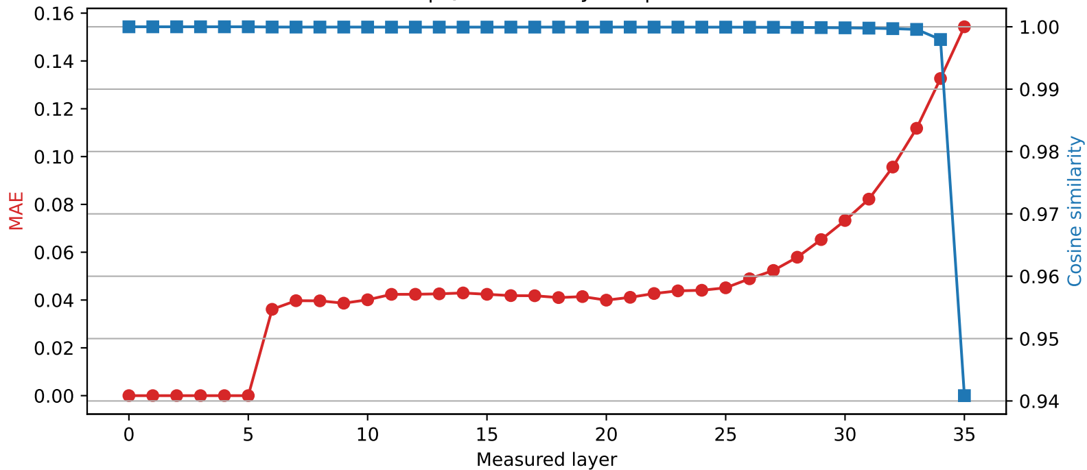
SmolLM3-3B | Quantized layer 5 | float32 \rightarrow int2
