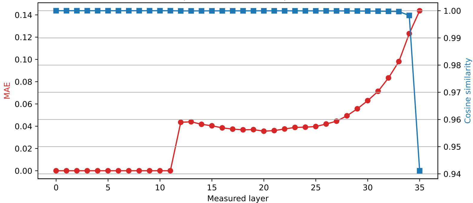
SmolLM3-3B | Quantized layer 11 | float32 \rightarrow int2
