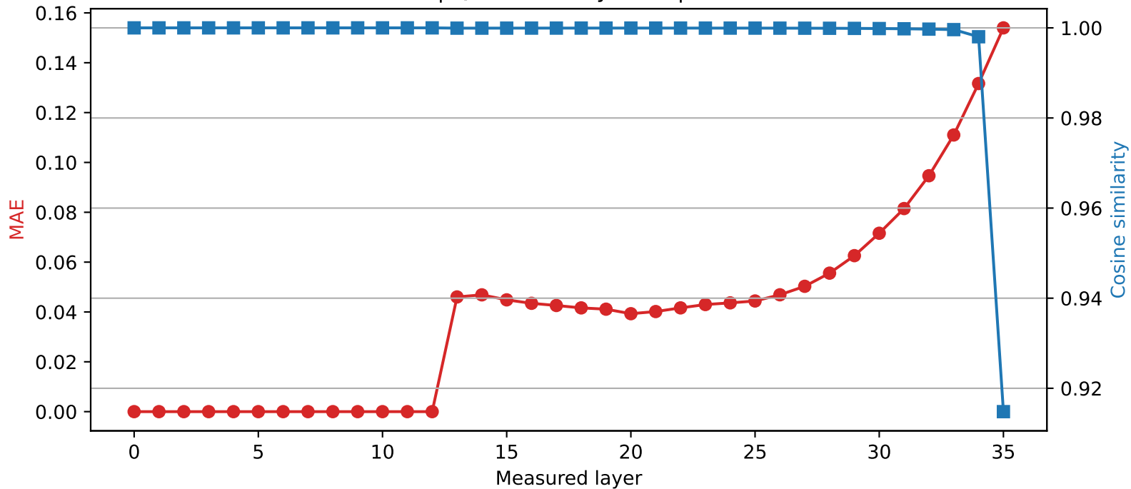
SmolLM3-3B | Quantized layer 12 | float32 \rightarrow int2
