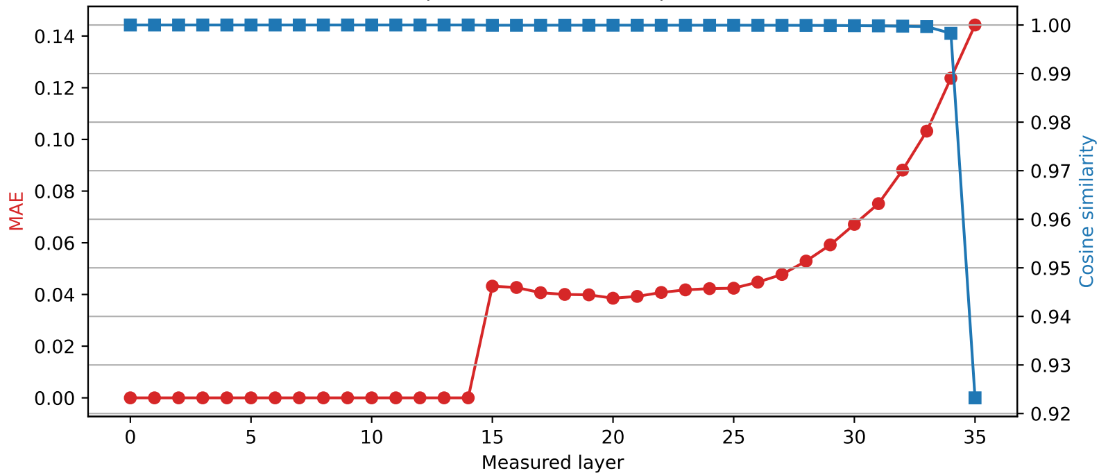
SmolLM3-3B | Quantized layer 14 | float32 \rightarrow int2
