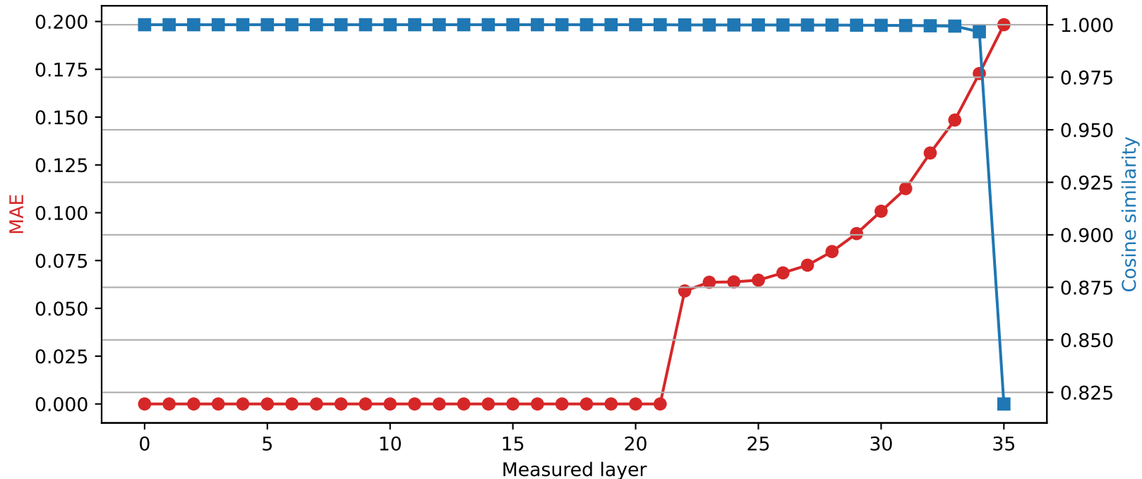
SmolLM3-3B | Quantized layer 21 | float32 \rightarrow int2
