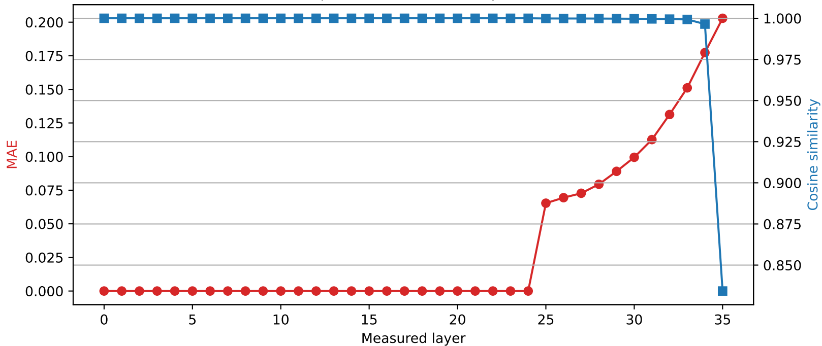
SmolLM3-3B | Quantized layer 24 | float32 \rightarrow int2
