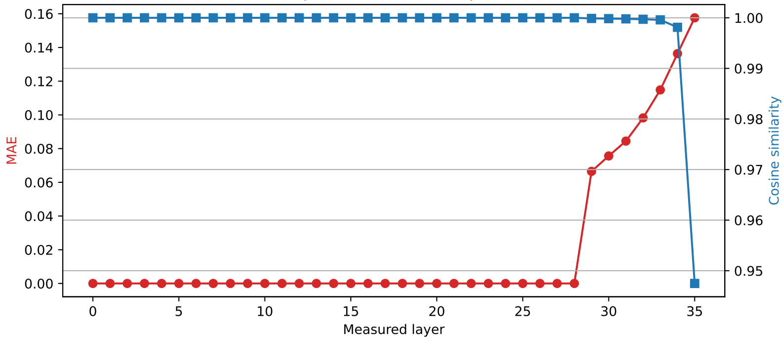
SmolLM3-3B | Quantized layer 28 | float32 \rightarrow int2
