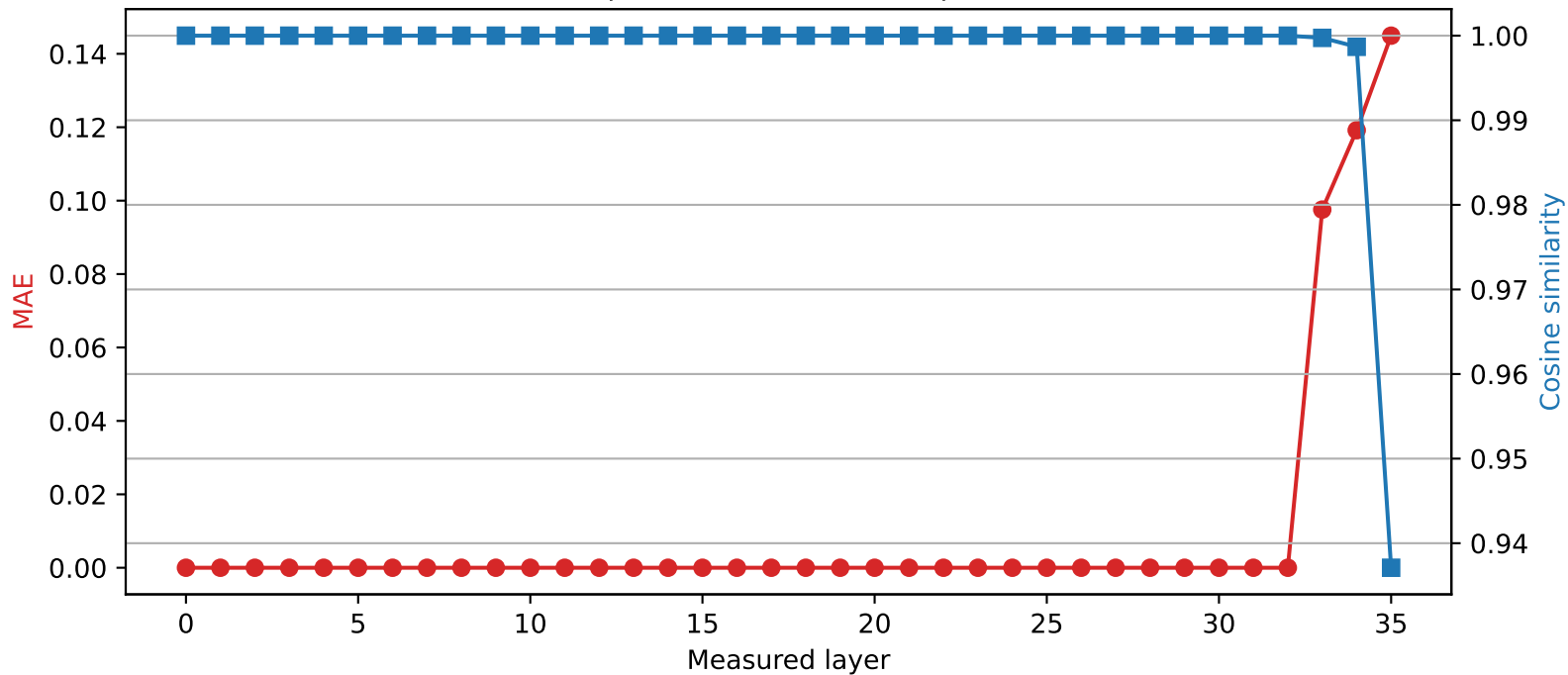
SmolLM3-3B | Quantized layer 32 | float32 → int2
