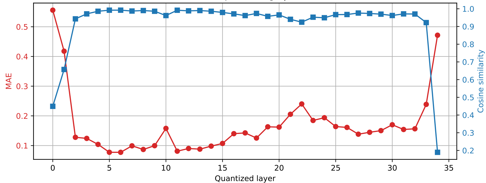
SmolLM3-3B | Prompt 2 Final RMSNorm output damage | float32 \rightarrow int2
