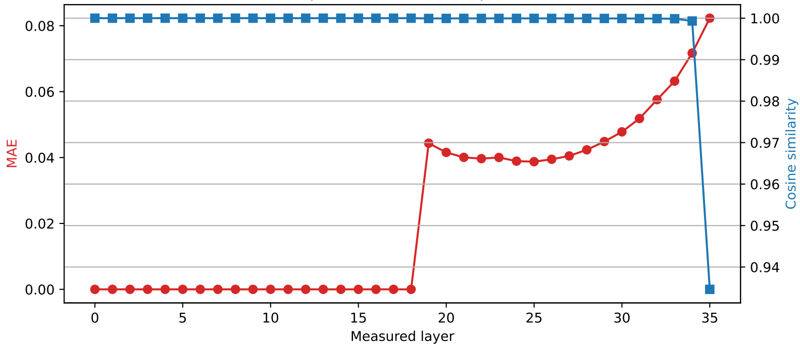
SmolLM3-3B | Quantized layer 18 | float32 → int2
