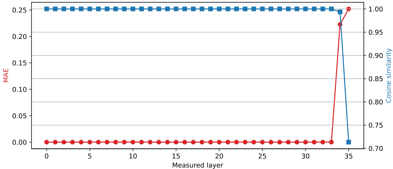
SmolLM3-3B | Quantized layer 33 | float32 \rightarrow int2
