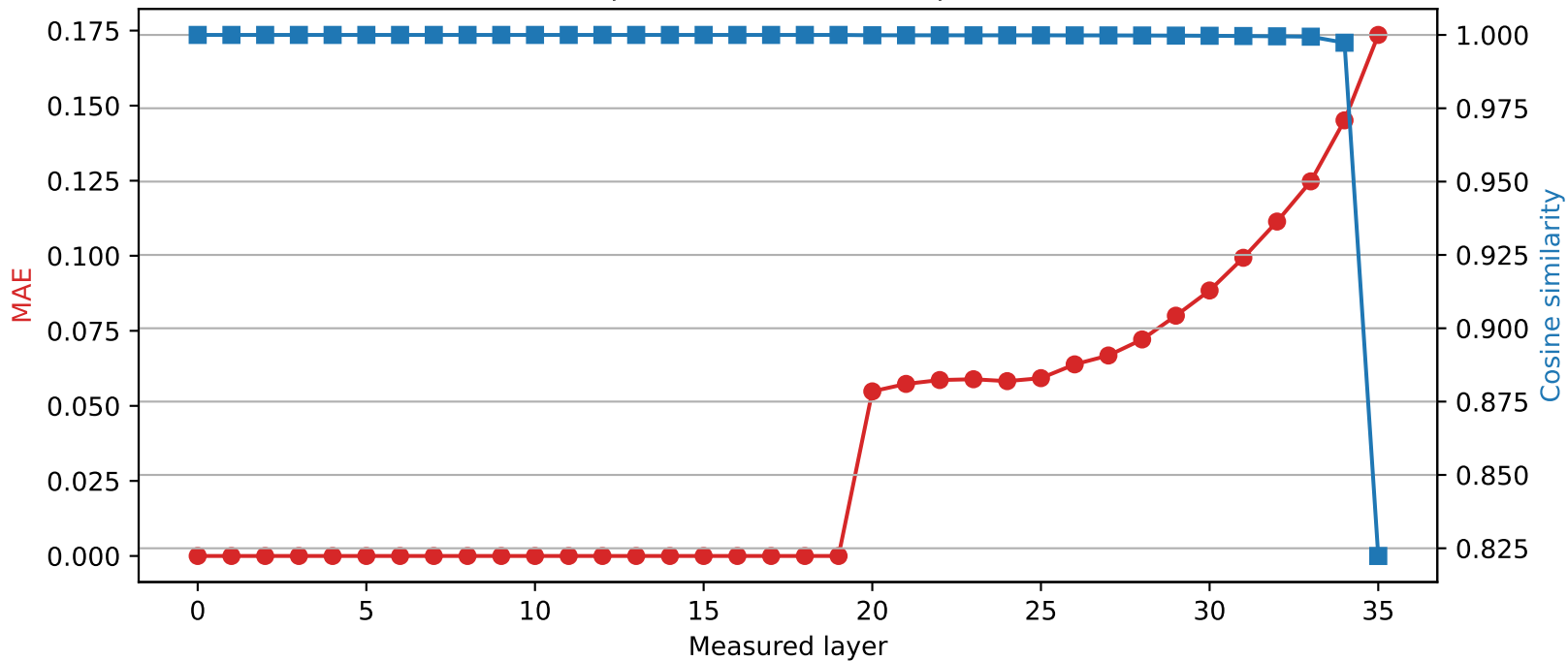
SmolLM3-3B | Quantized layer 19 | float32 → int2
