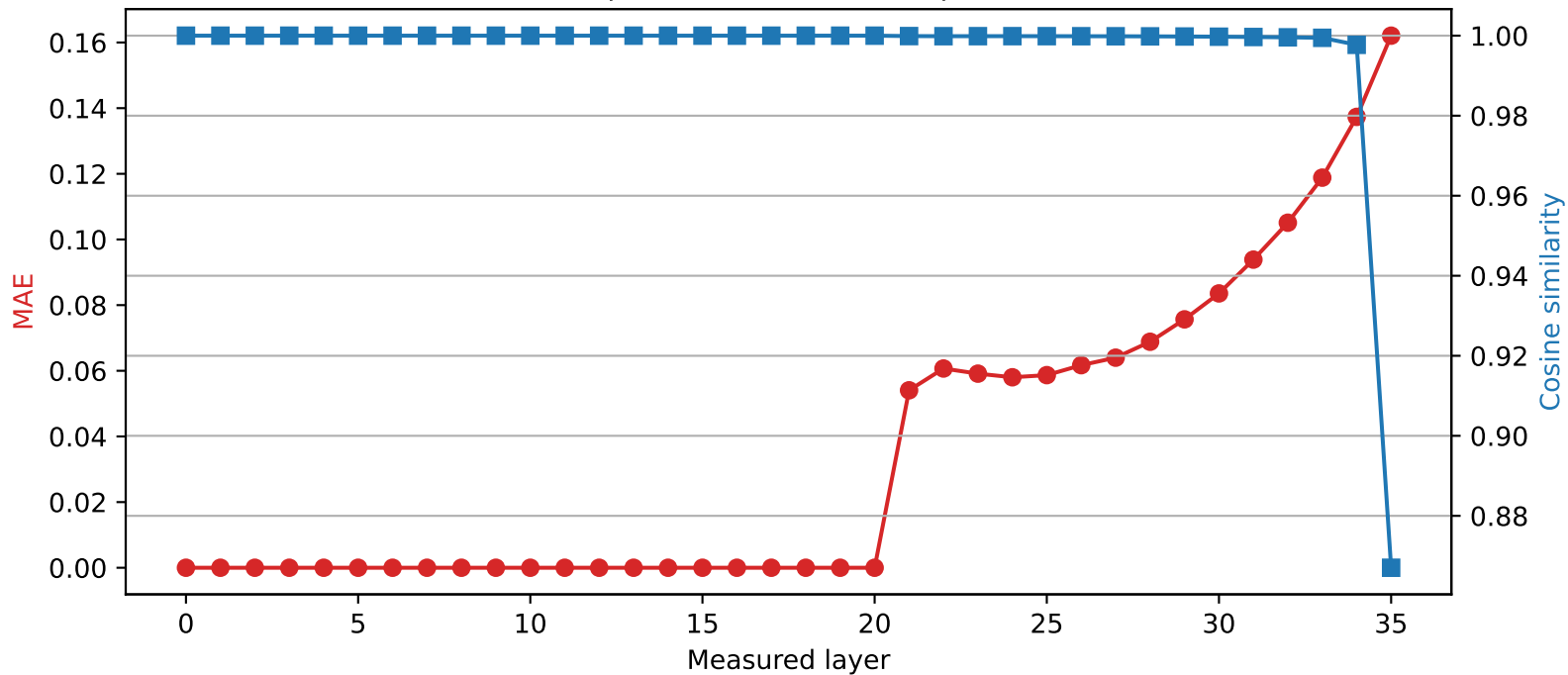
SmolLM3-3B | Quantized layer 20 | float32 \rightarrow int2
